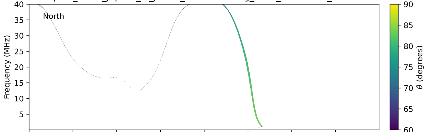
expres_earth_jupiter_io_jrm33_lossc-wid1deg_3kev_19940111_v11.cdf
