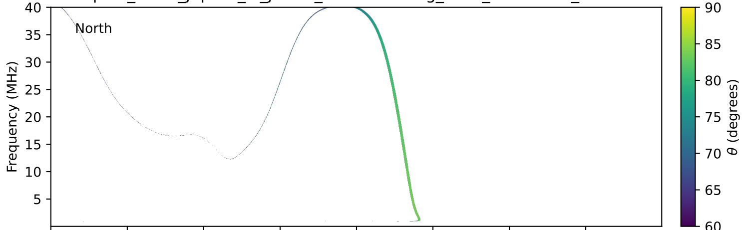
expres_earth_jupiter_io_jrm33_lossc-wid1deg_3kev_19940104_v11.cdf
