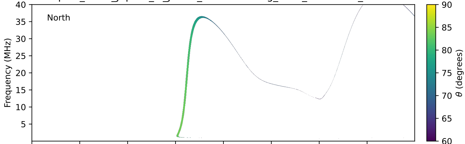
expres_earth_jupiter_io_jrm09_lossc-wid1deg_3kev_19940130_v11.cdf
