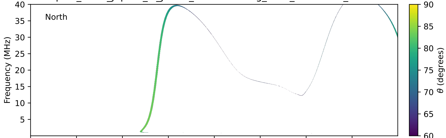
expres_earth_jupiter_io_jrm09_lossc-wid1deg_3kev_19940123_v11.cdf
