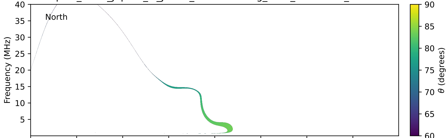
expres_earth_jupiter_io_jrm09_lossc-wid1deg_3kev_19940120_v11.cdf
