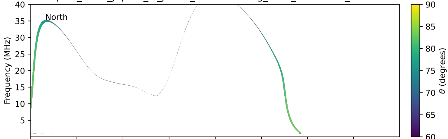
expres_earth_jupiter_io_jrm09_lossc-wid1deg_3kev_19940118_v11.cdf
