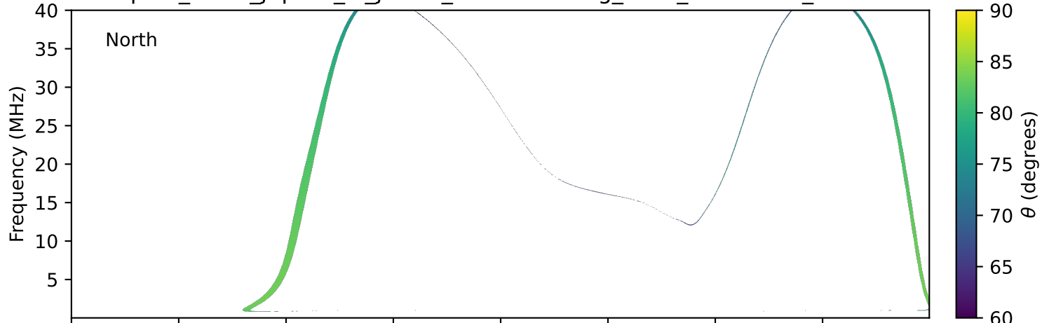
expres_earth_jupiter_io_jrm09_lossc-wid1deg_3kev_19940116_v11.cdf
