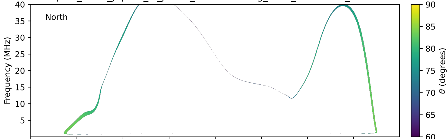
expres_earth_jupiter_io_jrm09_lossc-wid1deg_3kev_19940109_v11.cdf
