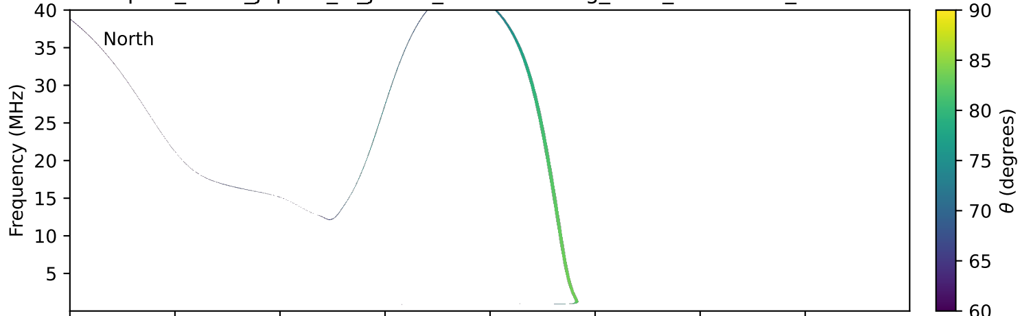
expres_earth_jupiter_io_jrm09_lossc-wid1deg_3kev_19940104_v11.cdf
