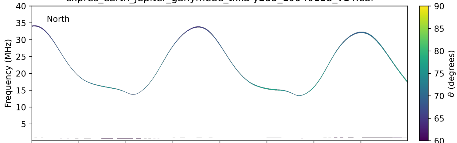
expres_earth_jupiter_ganymede_txka-y235_19940128_v14.cdf
