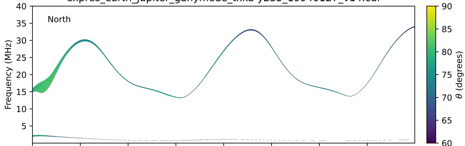
expres_earth_jupiter_ganymede_txka-y235_19940127_v14.cdf
