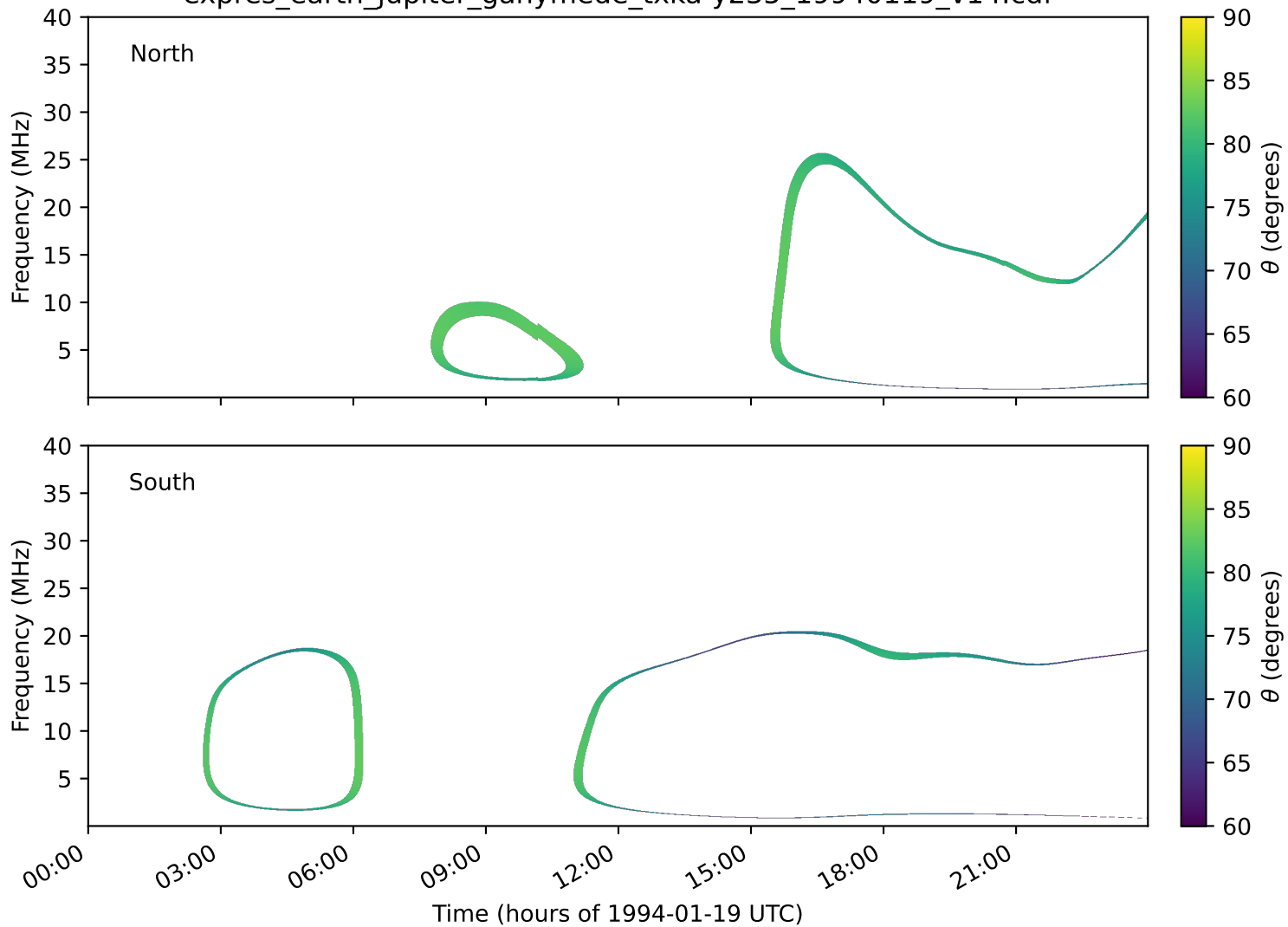
expres_earth_jupiter_ganymede_txka-y235_19940119_v14.cdf
