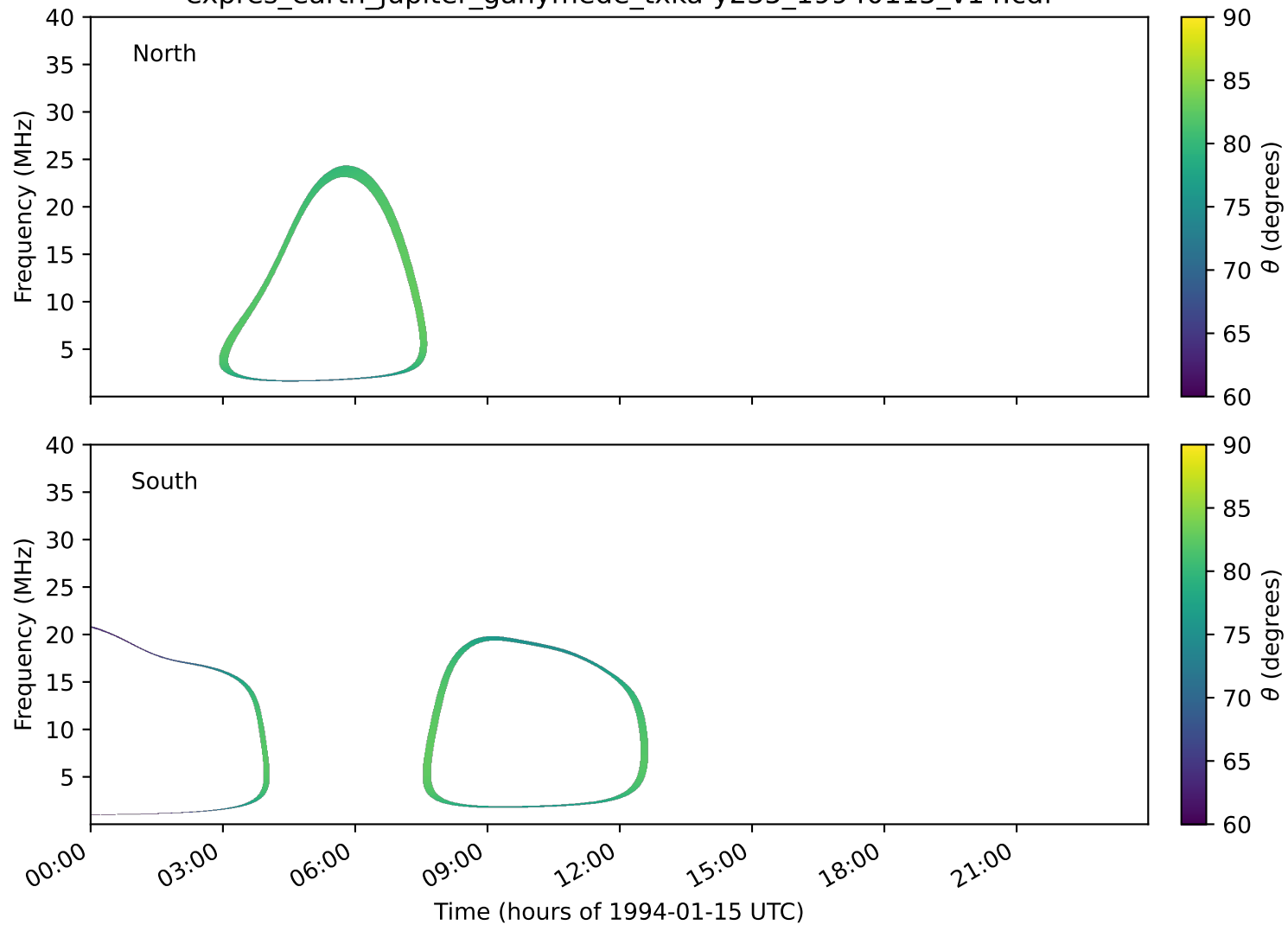
expres_earth_jupiter_ganymede_txka-y235_19940115_v14.cdf
