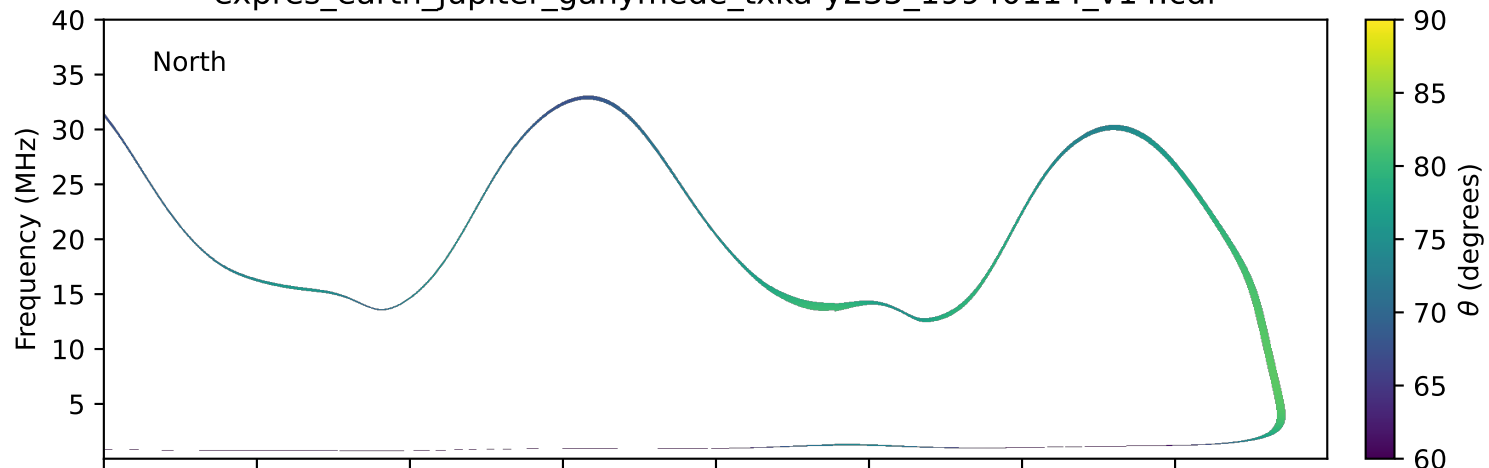
expres_earth_jupiter_ganymede_txka-y235_19940114_v14.cdf
