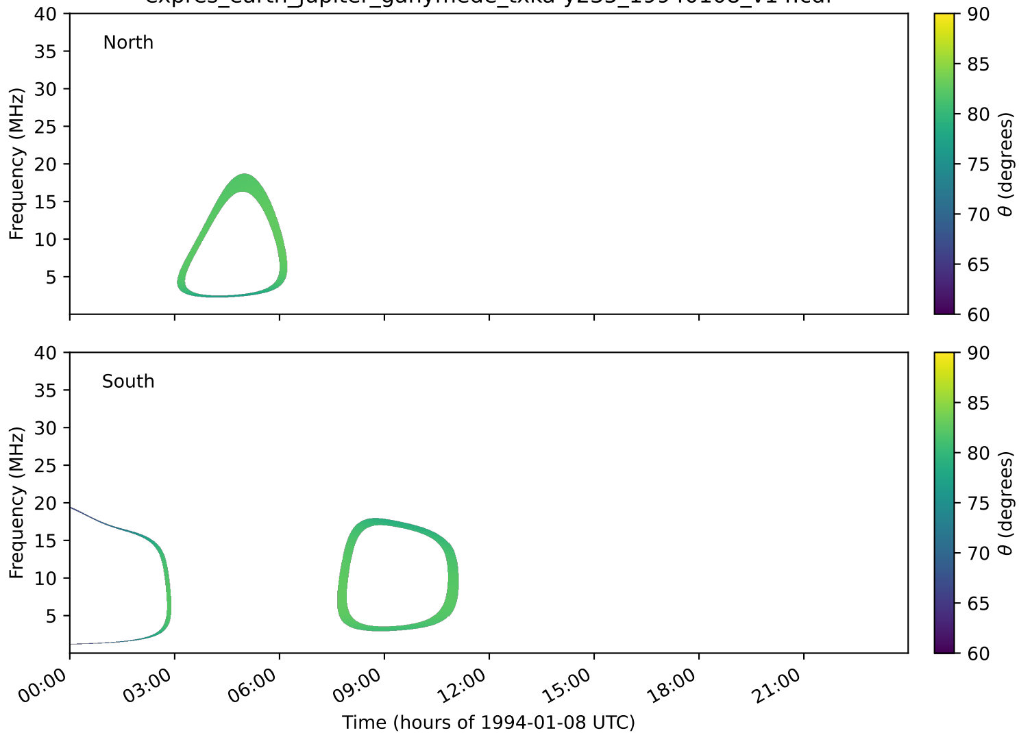
expres_earth_jupiter_ganymede_txka-y235_19940108_v14.cdf
