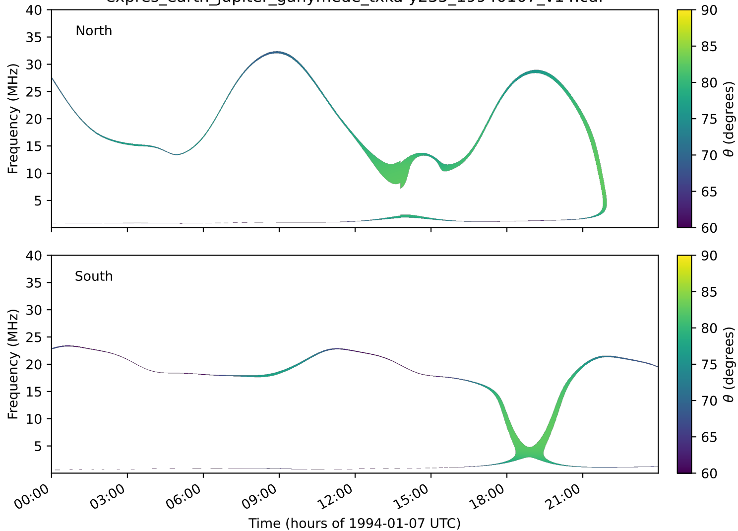
expres_earth_jupiter_ganymede_txka-y235_19940107_v14.cdf
