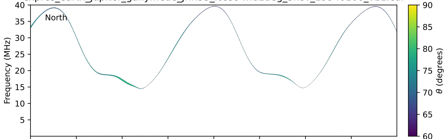
expres_earth_jupiter_ganymede_jrm33_lossc-wid1deg_3kev_19940106_v11.cdf
