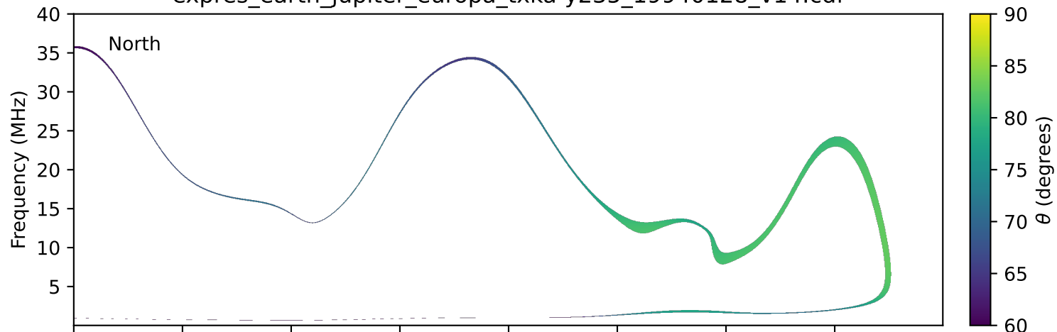
expres_earth_jupiter_europa_txka-y235_19940128_v14.cdf
