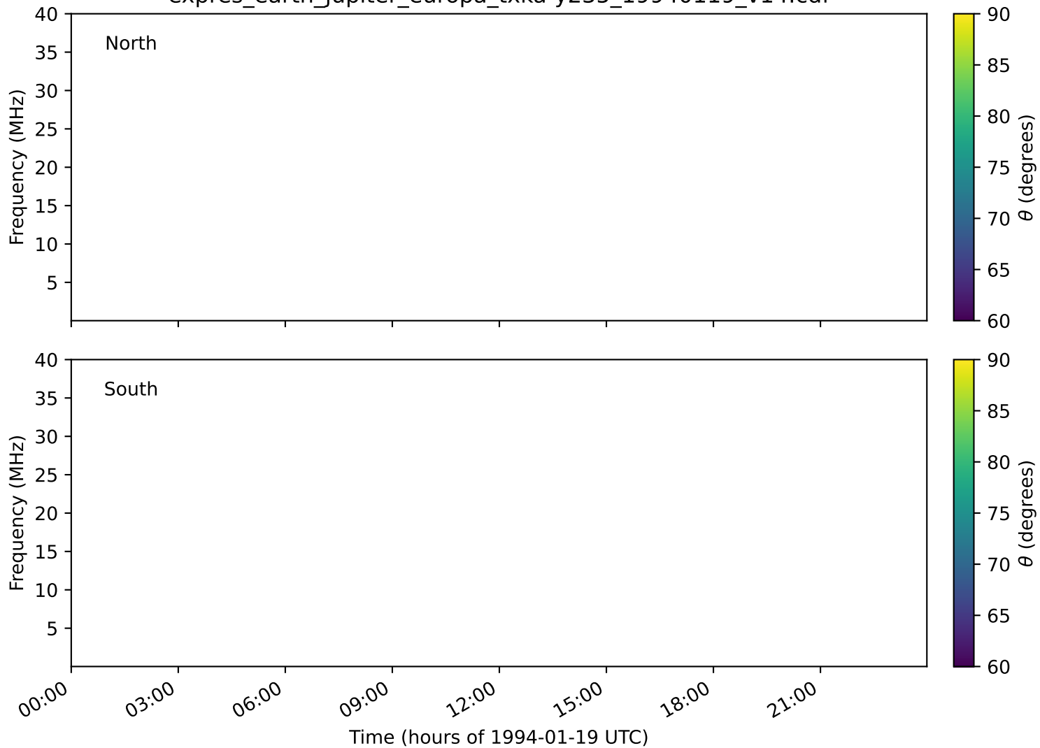
expres_earth_jupiter_europa_txka-y235_19940119_v14.cdf
