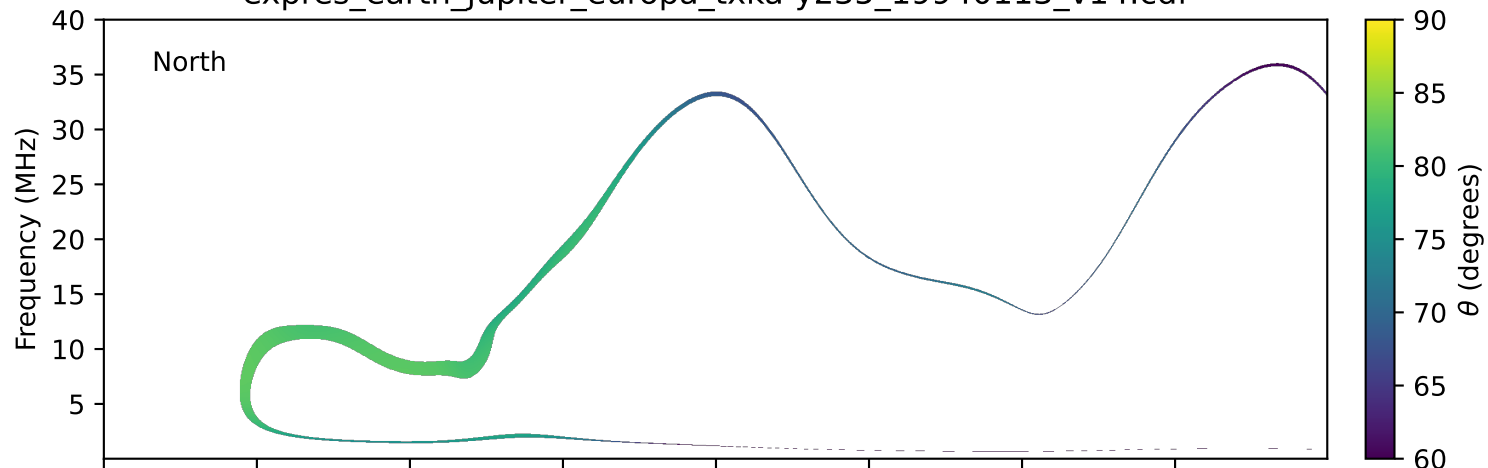
expres_earth_jupiter_europa_txka-y235_19940113_v14.cdf
