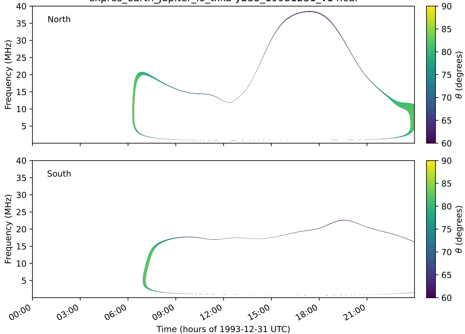
expres_earth_jupiter_io_txka-y235_19931231_v14.cdf
