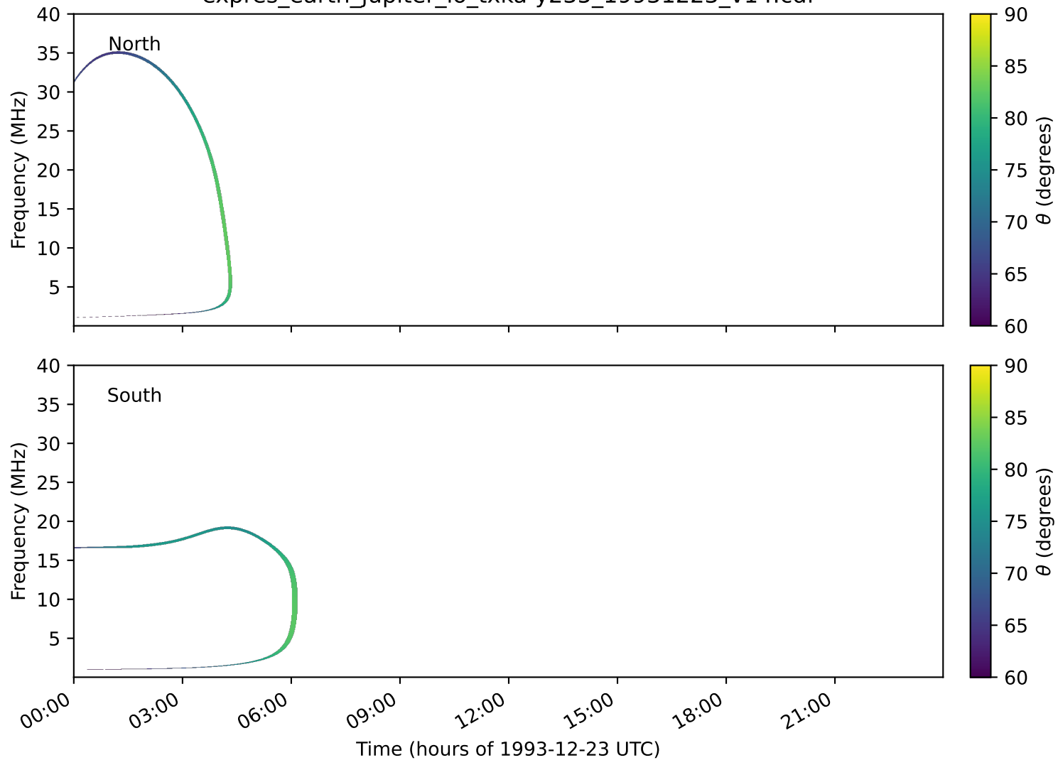
expres_earth_jupiter_io_txka-y235_19931223_v14.cdf
