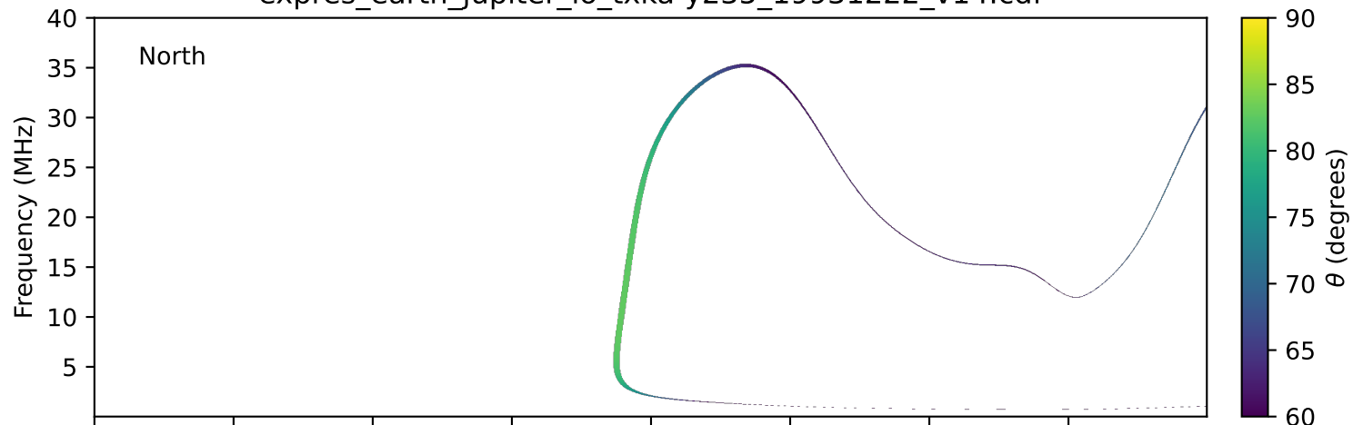
expres_earth_jupiter_io_txka-y235_19931222_v14.cdf
