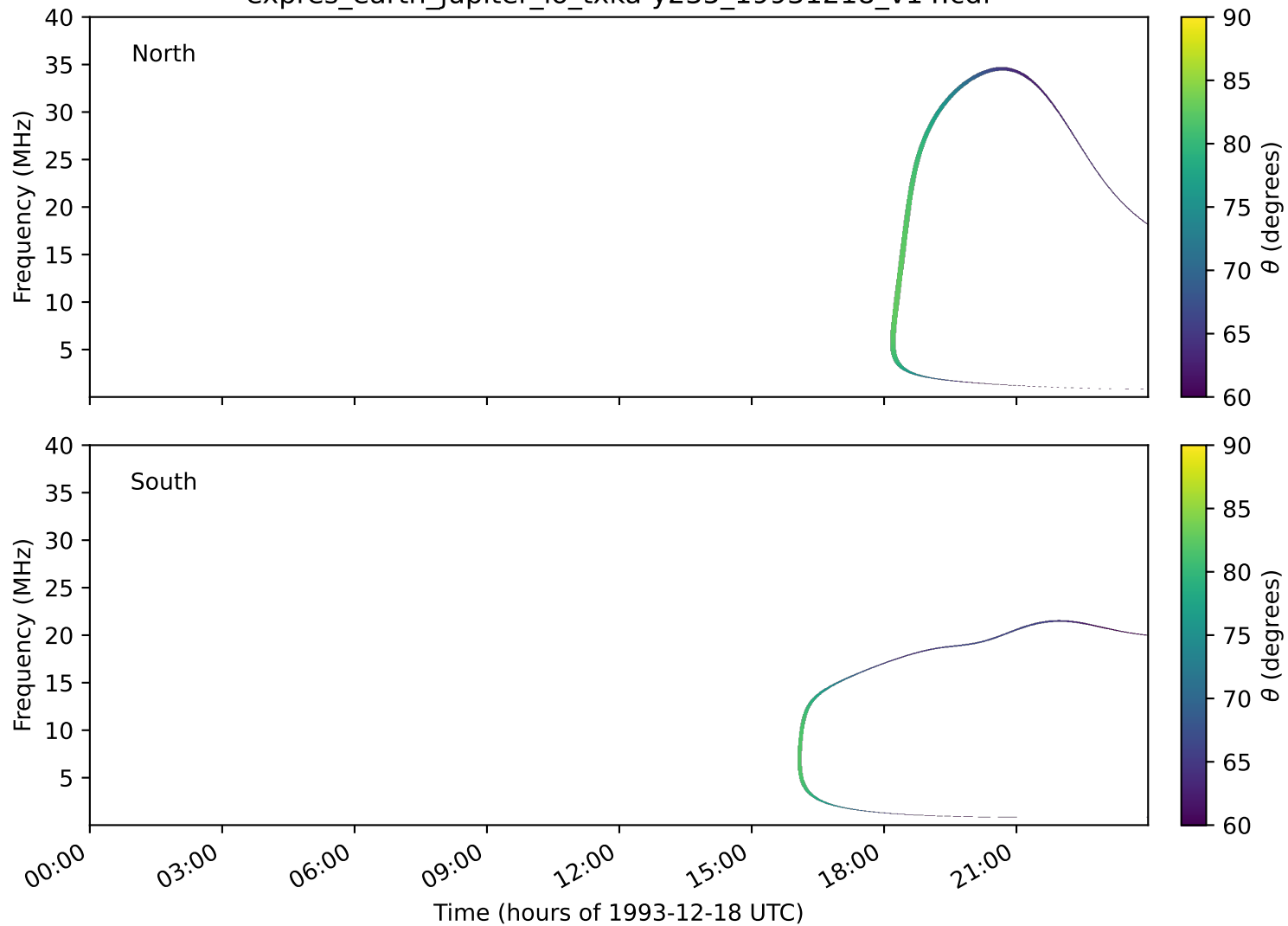
expres_earth_jupiter_io_txka-y235_19931218_v14.cdf
