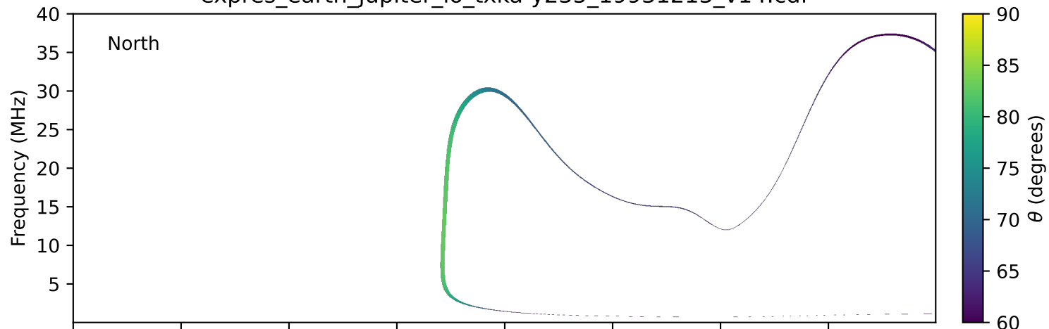
expres_earth_jupiter_io_txka-y235_19931213_v14.cdf
