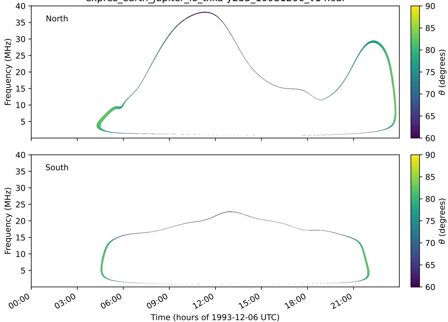
expres_earth_jupiter_io_txka-y235_19931206_v14.cdf
