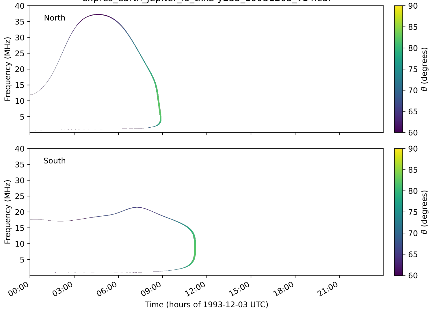
expres_earth_jupiter_io_txka-y235_19931203_v14.cdf
