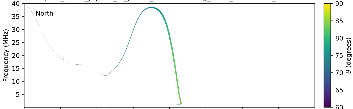
expres_earth_jupiter_io_jrm33_lossc-wid1deg_3kev_19931228_v11.cdf
