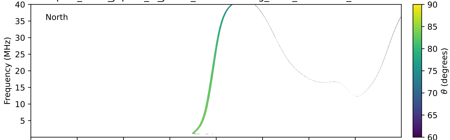
expres_earth_jupiter_io_jrm33_lossc-wid1deg_3kev_19931222_v11.cdf
