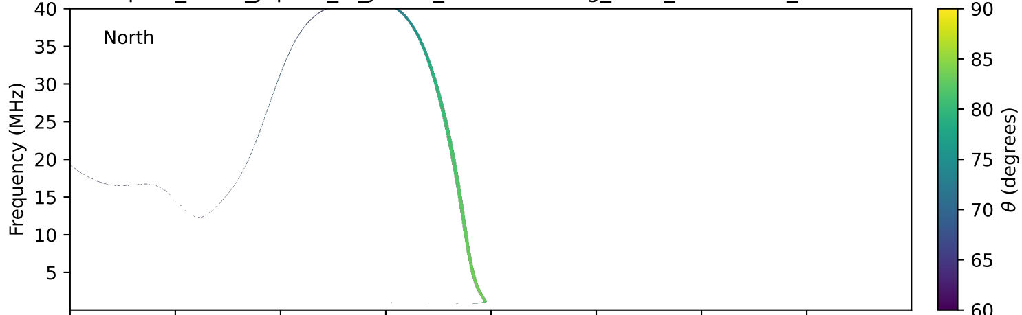
expres_earth_jupiter_io_jrm33_lossc-wid1deg_3kev_19931219_v11.cdf
