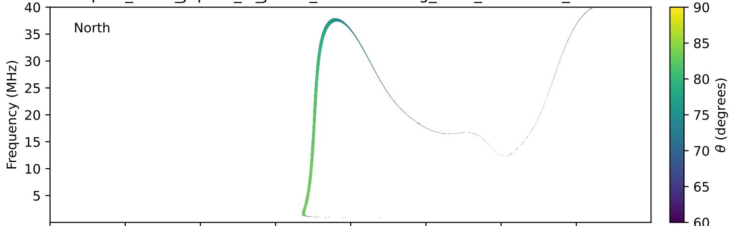
expres_earth_jupiter_io_jrm33_lossc-wid1deg_3kev_19931213_v11.cdf
