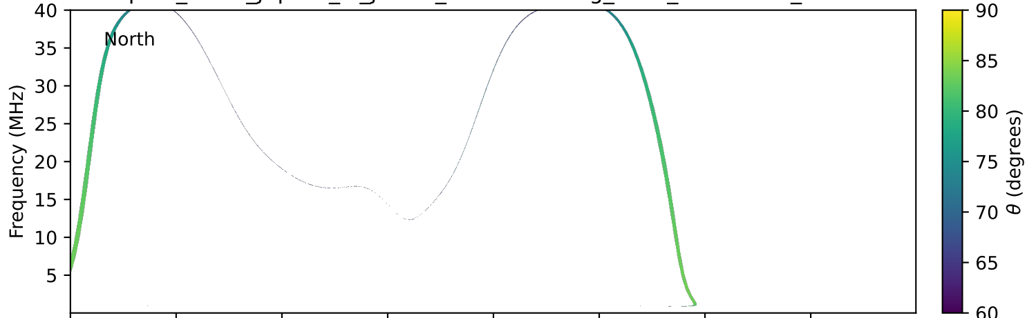
expres_earth_jupiter_io_jrm33_lossc-wid1deg_3kev_19931208_v11.cdf
