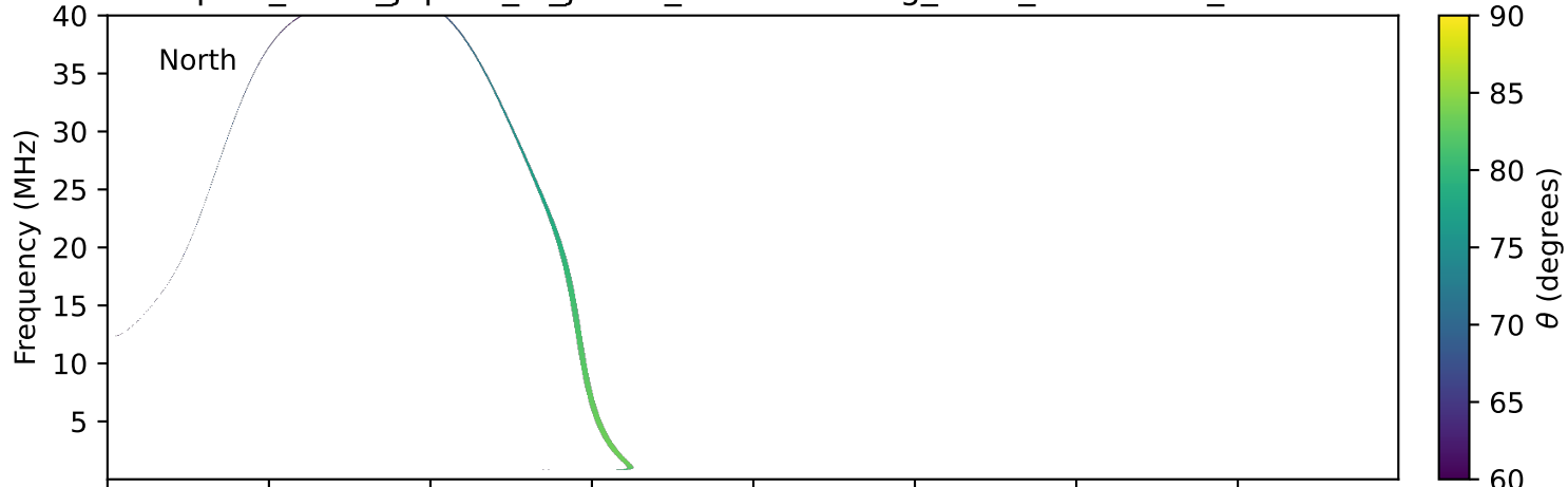
expres_earth_jupiter_io_jrm33_lossc-wid1deg_3kev_19931203_v11.cdf
