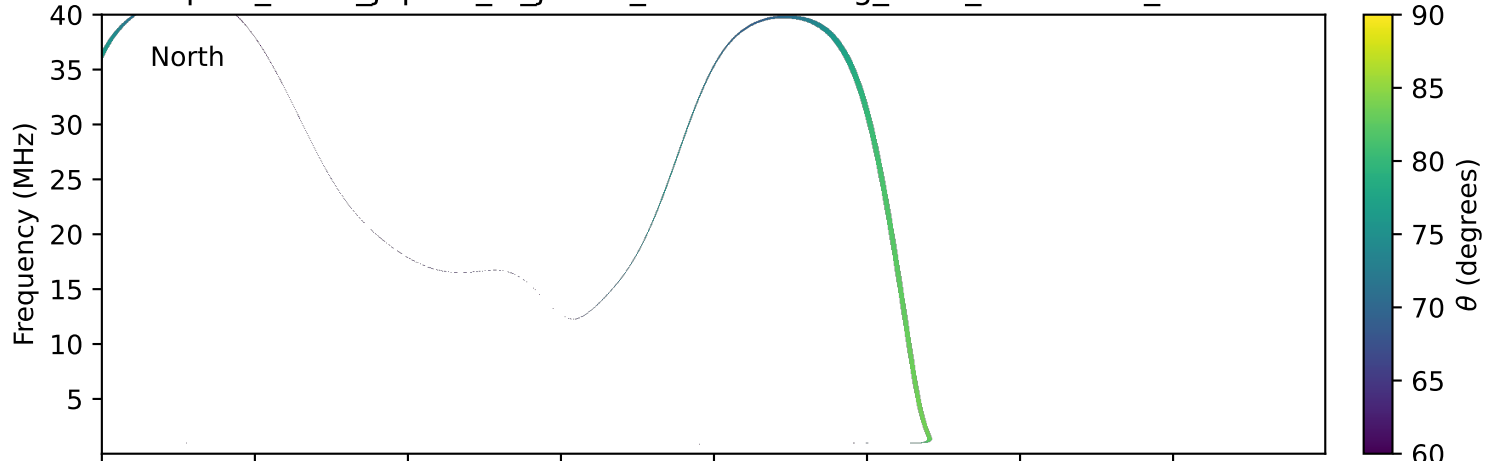
expres_earth_jupiter_io_jrm33_lossc-wid1deg_3kev_19931201_v11.cdf
