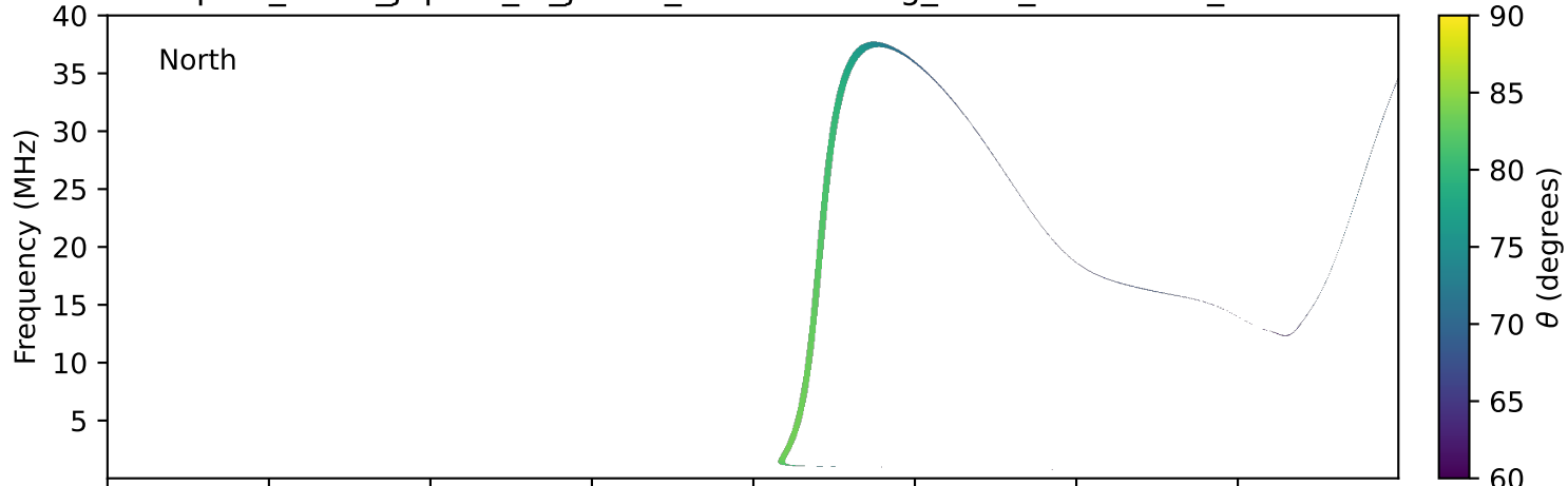
expres_earth_jupiter_io_jrm09_lossc-wid1deg_3kev_19931229_v11.cdf
