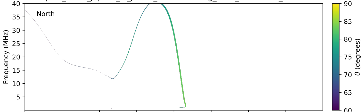
expres_earth_jupiter_io_jrm09_lossc-wid1deg_3kev_19931228_v11.cdf
