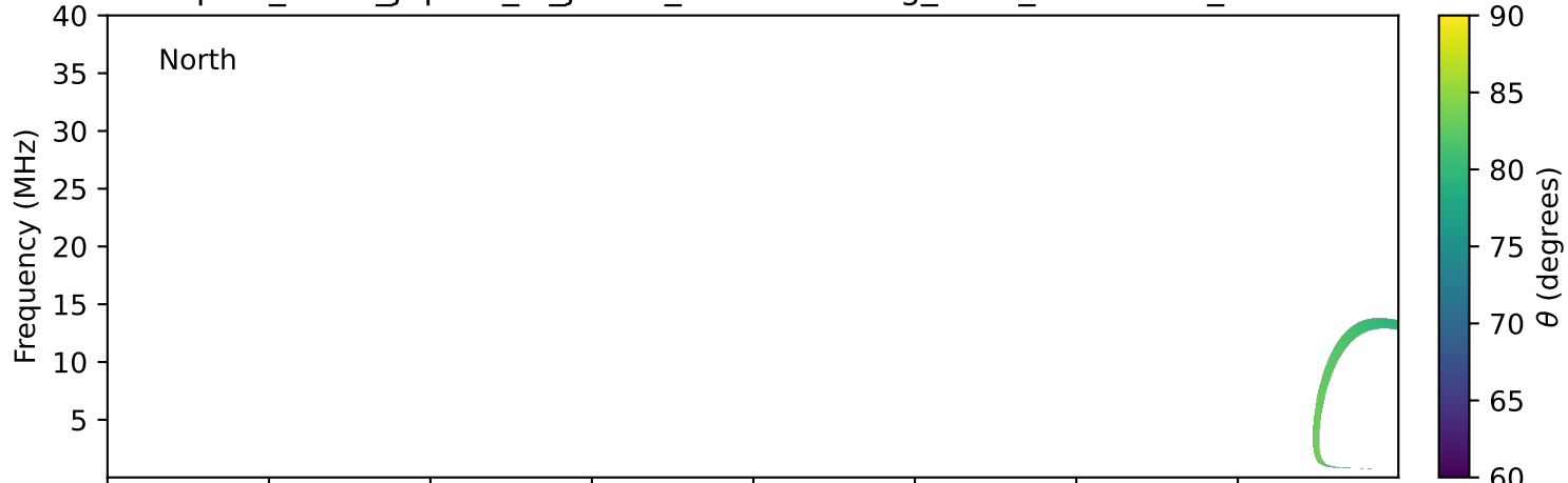
expres_earth_jupiter_io_jrm09_lossc-wid1deg_3kev_19931225_v11.cdf
