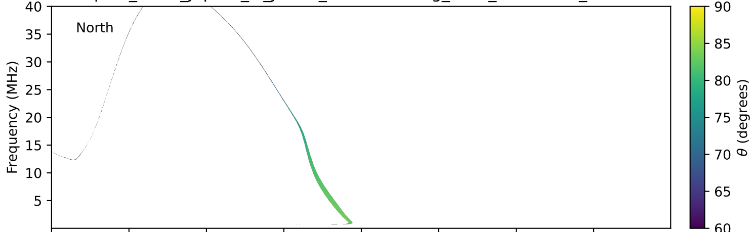
expres_earth_jupiter_io_jrm09_lossc-wid1deg_3kev_19931210_v11.cdf
