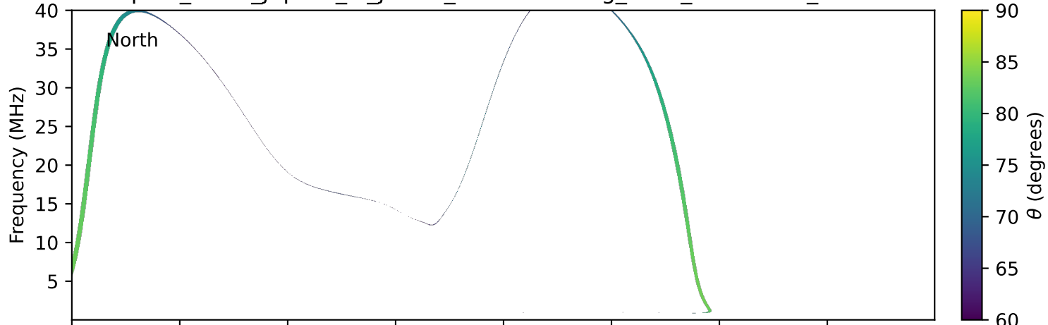
expres_earth_jupiter_io_jrm09_lossc-wid1deg_3kev_19931208_v11.cdf
