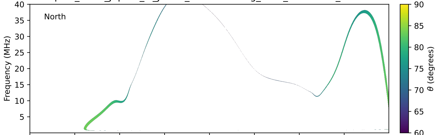
expres_earth_jupiter_io_jrm09_lossc-wid1deg_3kev_19931206_v11.cdf
