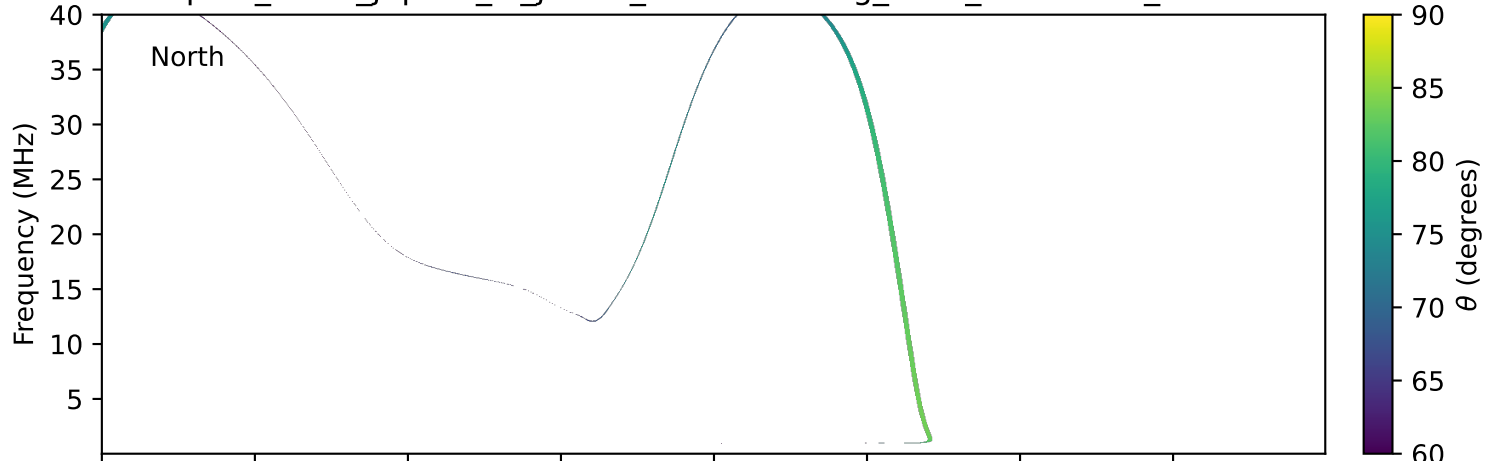
expres_earth_jupiter_io_jrm09_lossc-wid1deg_3kev_19931201_v11.cdf
