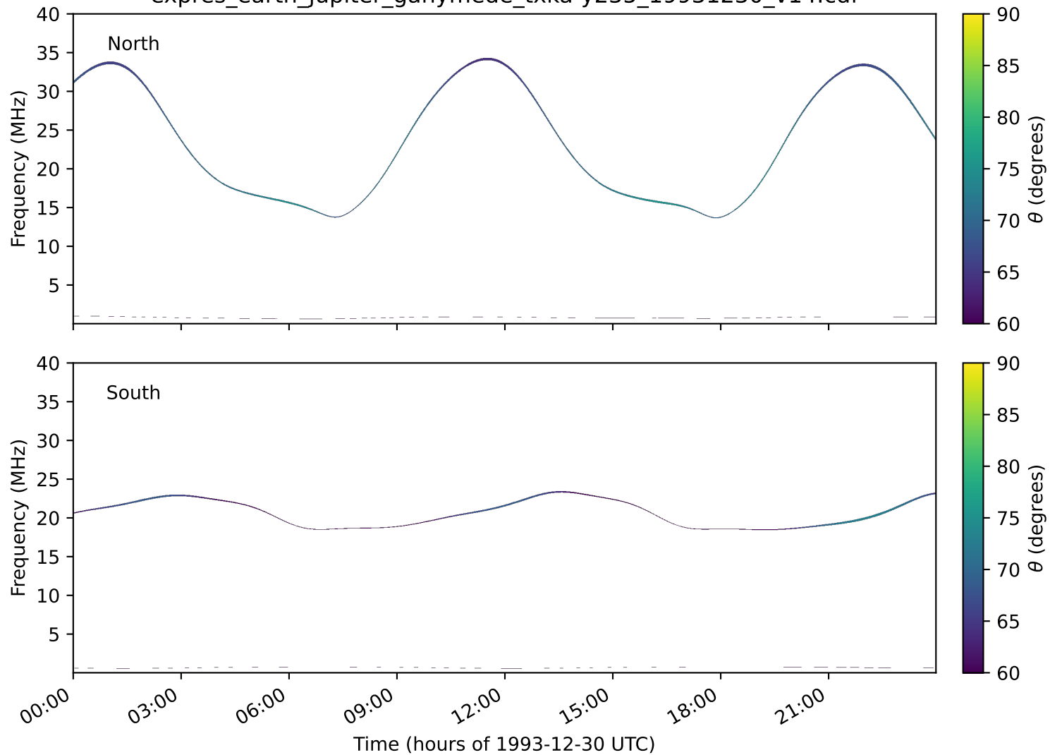
expres_earth_jupiter_ganymede_txka-y235_19931230_v14.cdf
