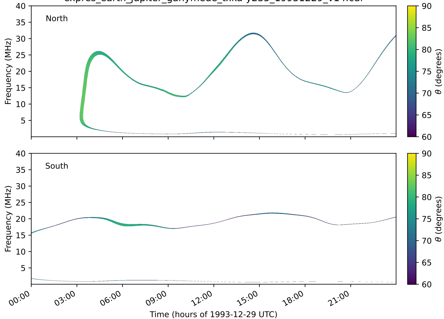
expres_earth_jupiter_ganymede_txka-y235_19931229_v14.cdf
