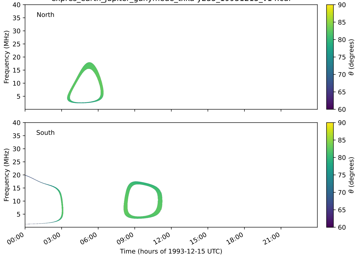
expres_earth_jupiter_ganymede_txka-y235_19931215_v14.cdf
