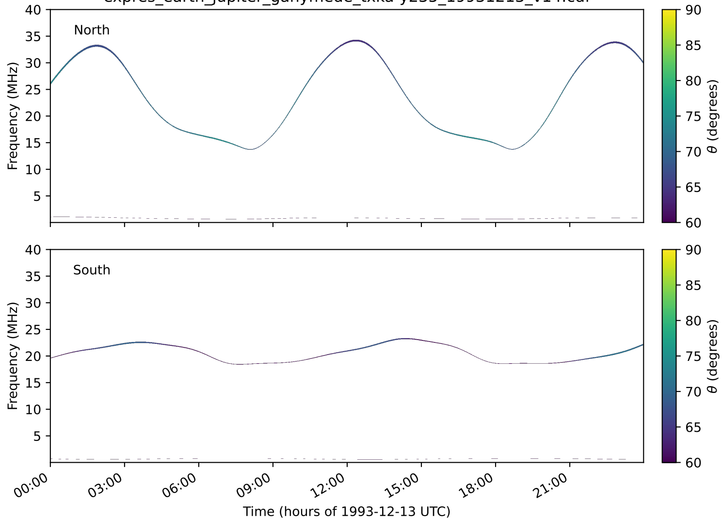
expres_earth_jupiter_ganymede_txka-y235_19931213_v14.cdf
