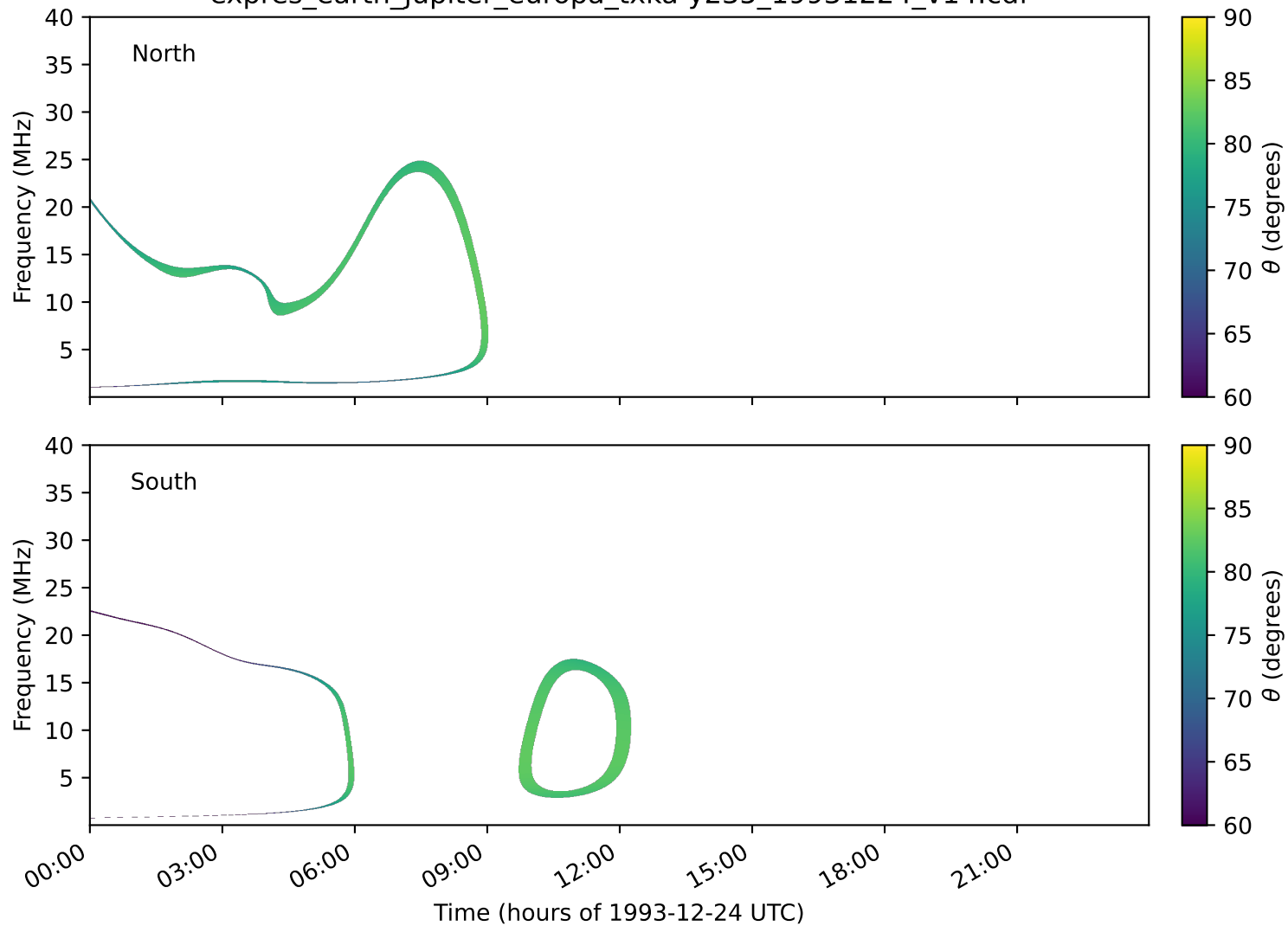
expres_earth_jupiter_europa_txka-y235_19931224_v14.cdf
