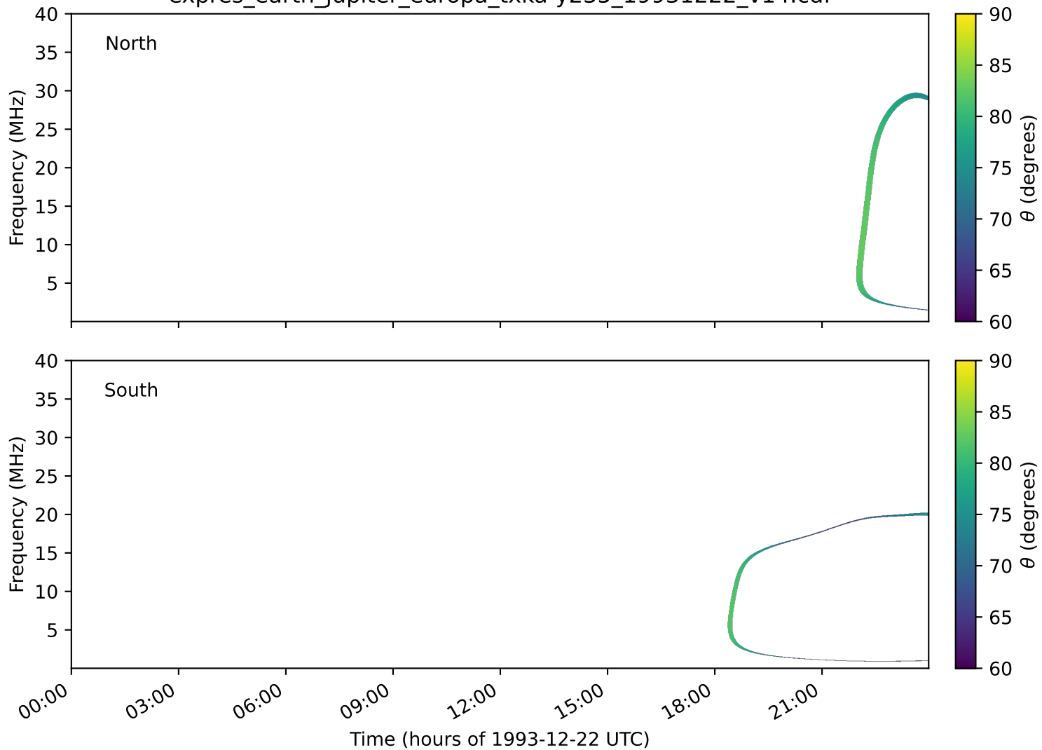
expres_earth_jupiter_europa_txka-y235_19931222_v14.cdf
