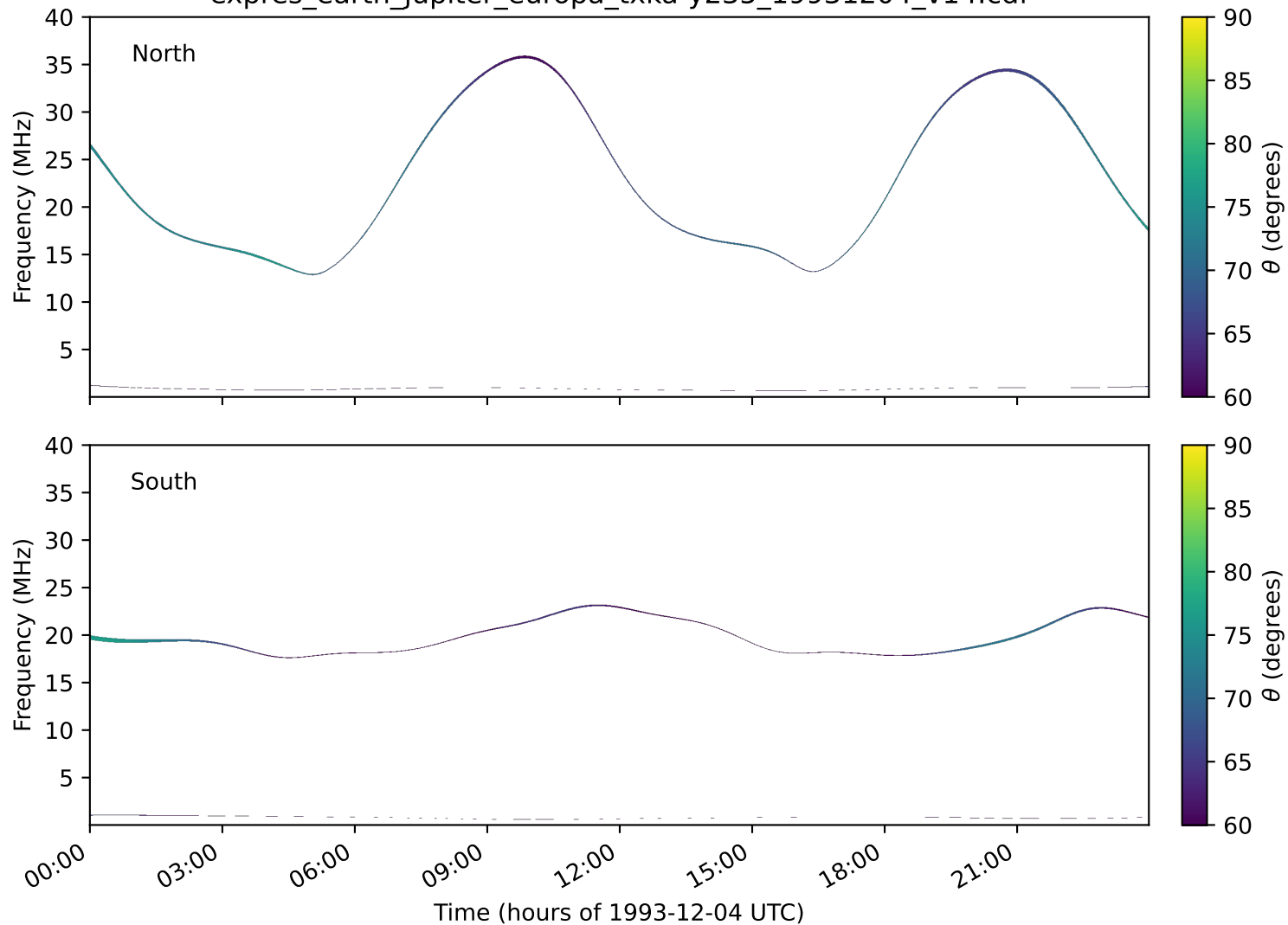
expres_earth_jupiter_europa_txka-y235_19931204_v14.cdf
