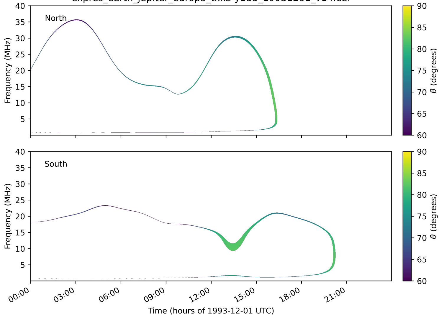
expres_earth_jupiter_europa_txka-y235_19931201_v14.cdf
