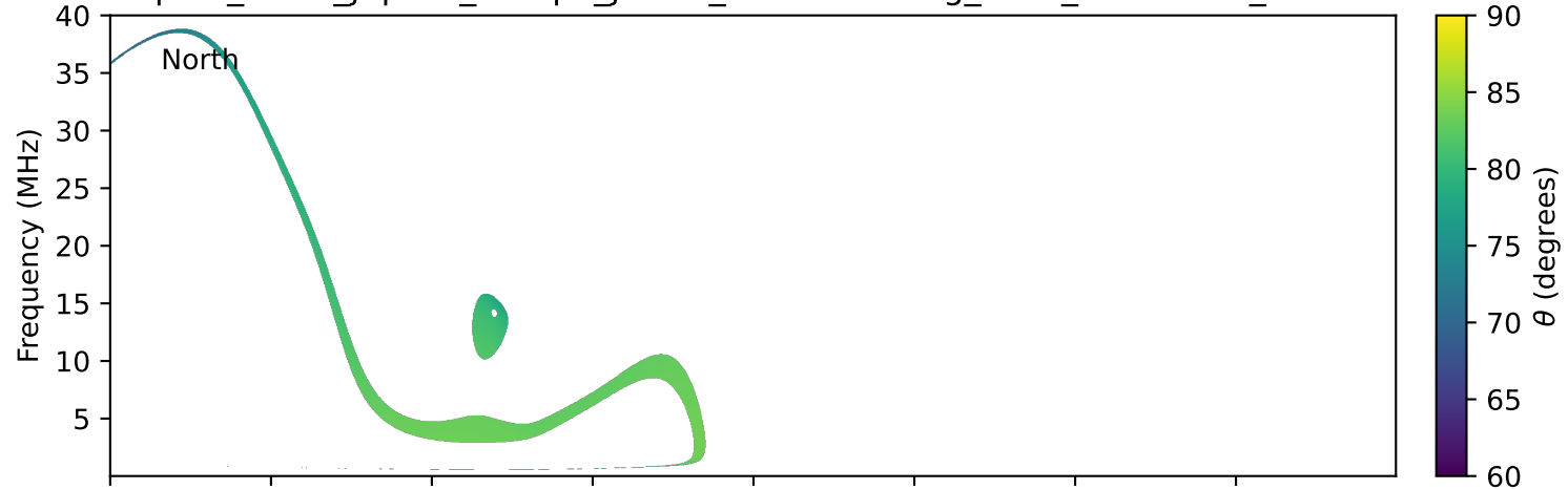
expres_earth_jupiter_europa_jrm33_lossc-wid1deg_3kev_19931216_v11.cdf
